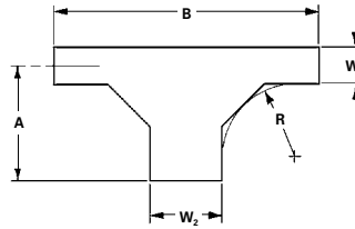
Mitered
