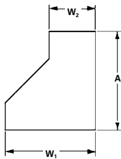
Right Reducer
